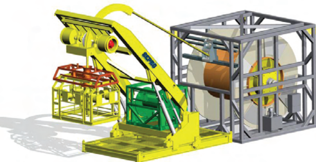
Subsea Tree Installation Workover Control System (IWOC)
