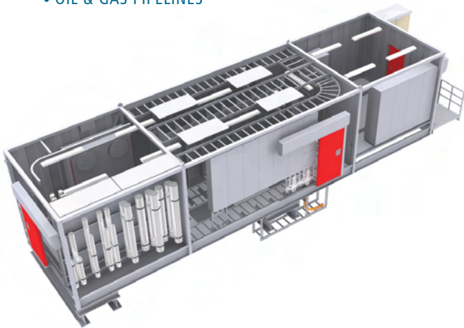
Integrated Wellhead Control System, HPU & Control Room
